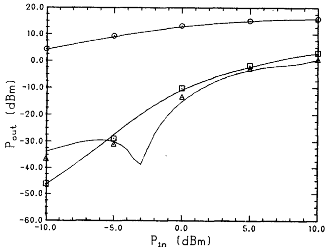
Fig. 6. Agreement between the (Materka) model responses and the measurements from Texas Instruments at fundamental frequency 0.2 GHz, and bias point V_{GB} = -0.373 V and V_{DB} = 2 V. (This bias point has been included in the optimization.) Solid lines represent computed model responses. Circles, triangles, and squares denote fundamental, second harmonic, and third harmonic measurements, respectively.
